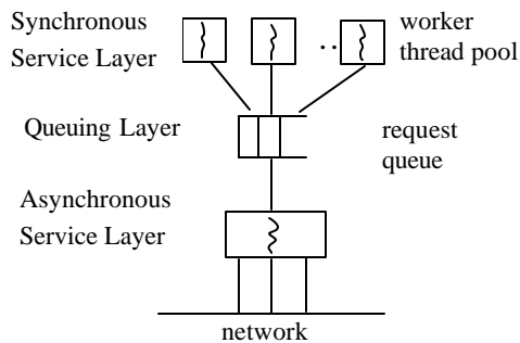
Figure 1. Structure of the Half-Sync/Half-Async Pattern
