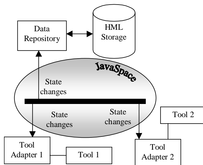
Figure 1: Holmes architecture
