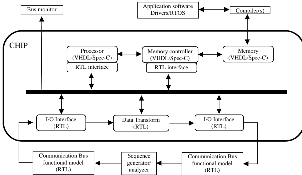
Figure 5: SoC Components specifications from [Keating and Bricaud 1999]
