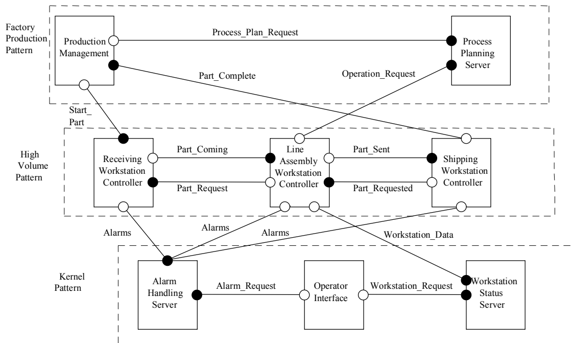
Figure 2: Software Architecture Diagram for the High Volume Target System
