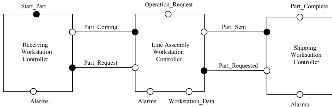
Figure 1: Software Architecture Diagram for High Volume Architectural Pattern
