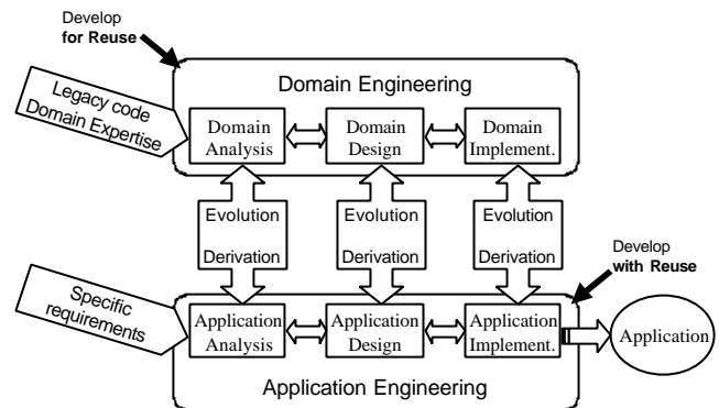
Figure 1 – The product line approach (inspired from STARS [1])
