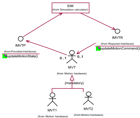
Figure 7: Part of the context diagram.
