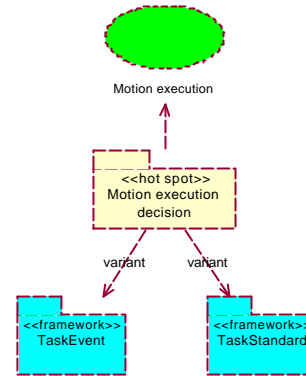
Figure 10: Managing variability with UML hot spots.
