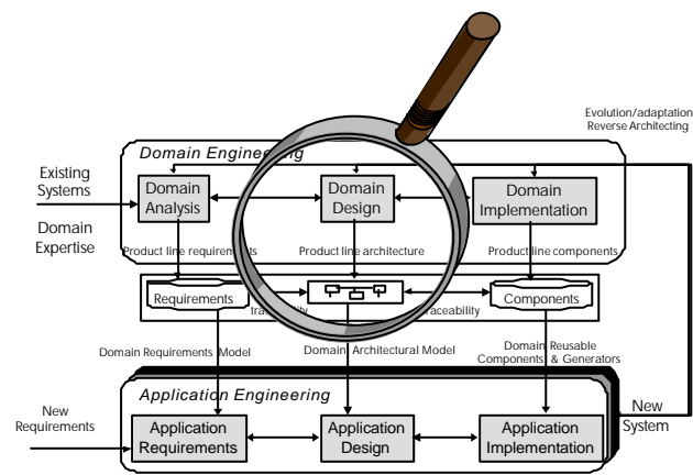
Figure 3: Product-line process extracted from [4].
