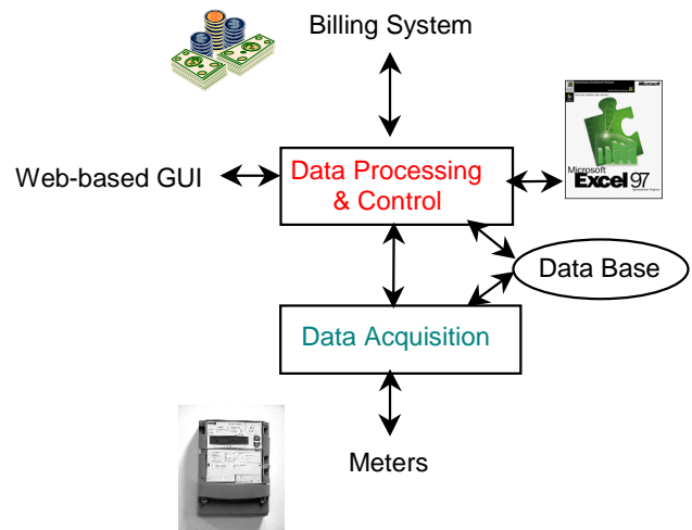
Figure 1. Athena conceptual architecture.
