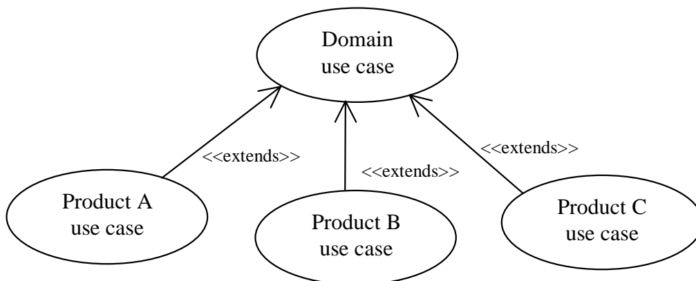
Figure 2: Domain use case as generalization of product use cases
