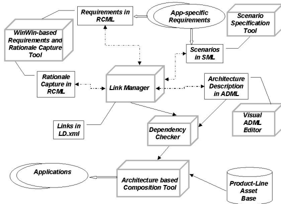
Figure 5. Prototype Tool Suite for Product Line Development
