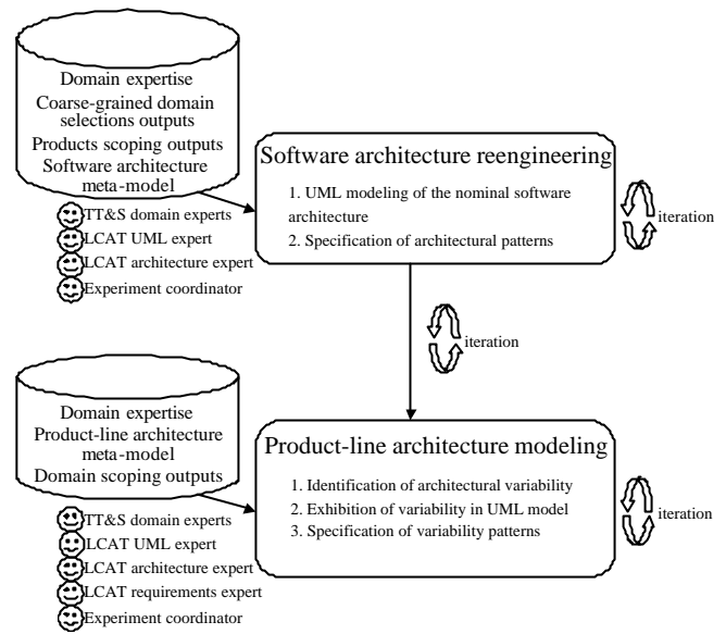
Figure 4: Product-line architecture design process in Thomson-CSF experiment.
