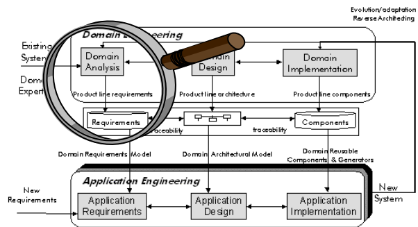
Figure 2: Product line process extracted from [8].
