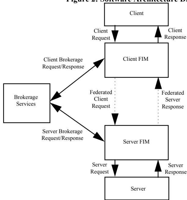
Figure 2: Software Architecture Diagram for the High Volume Target System
