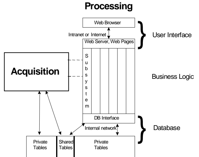
Figure 4. Three-tiered architecture.
