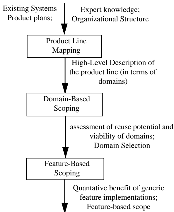
Figure 2. Solution Components
