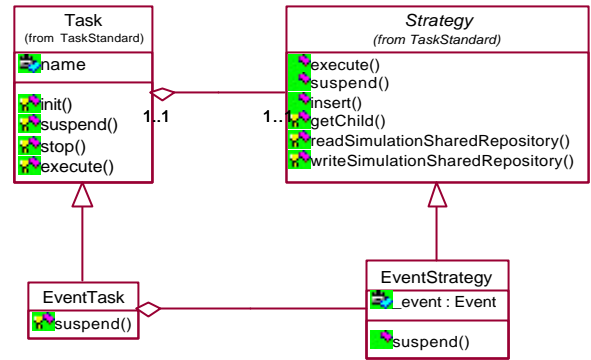
Figure 8: The TaskEvent framework in UML.
