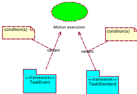
Figure 9: Representing variability in the UML model
