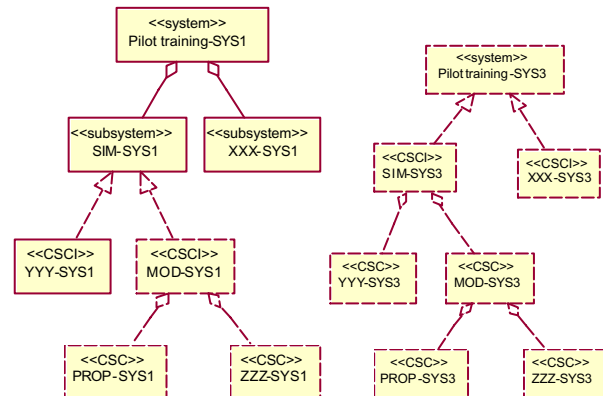
Figure 5: Comparison of referential use between systems
