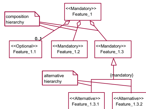
Figure 10: Features attributes and relationships according to FODA.
