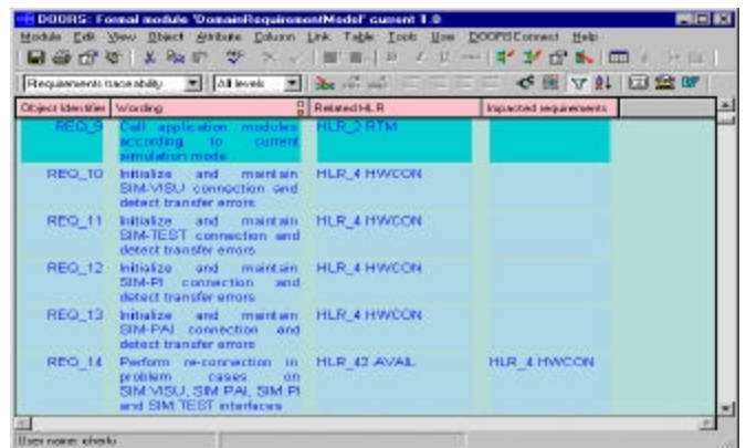
Figure 9: Doors “requirements traceability” view of domain requirements model.
