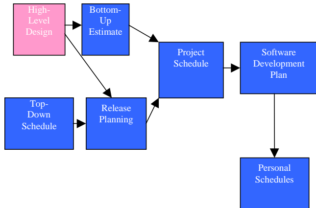
Figure 3. Architecture-centered software project planning.
