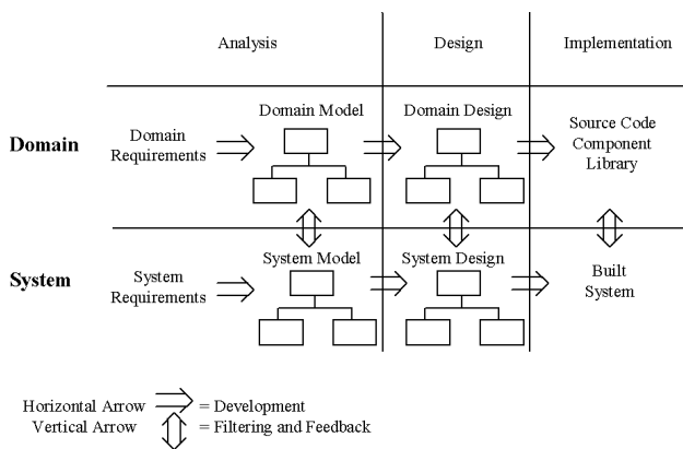
Figure 1. Product Line Engineering Process Model
