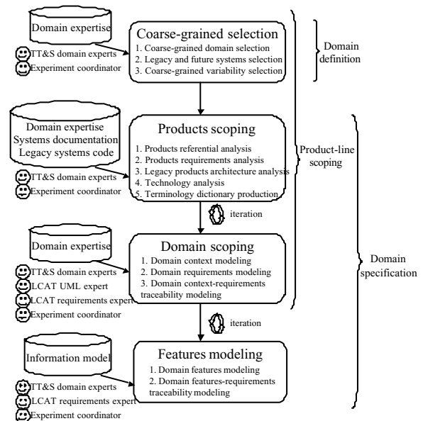
Figure 3: Domain analysis process part in Thomson-CSF experiment.
