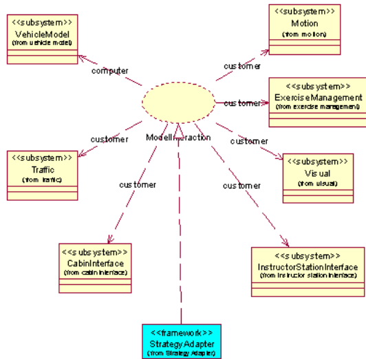
Figure 11: Variability framework realizing the model interaction collaboration.
