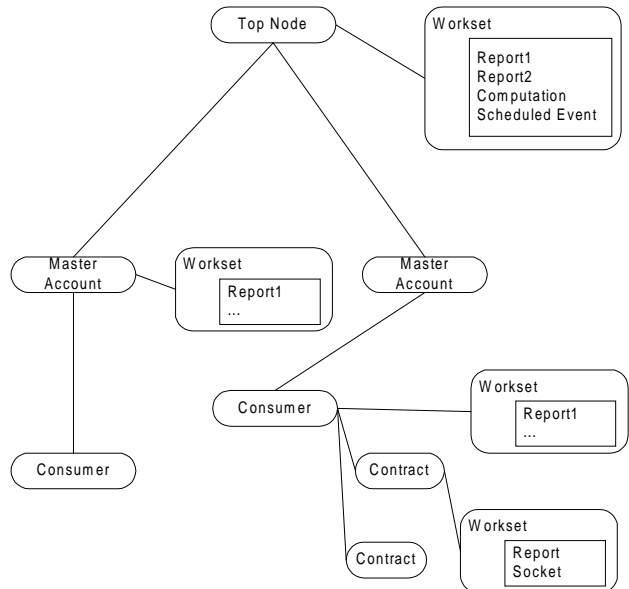
Figure 5. Consumer tree.
