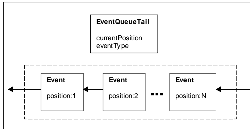
Figure 2: Event Queue
