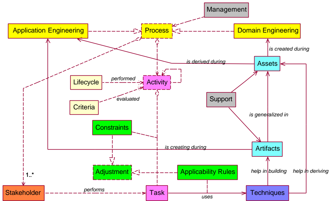
Figure 2 – PLPF - Product Line Process meta-model
