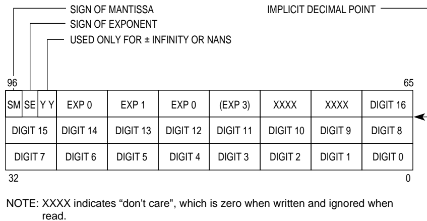
Figure 1-11. Packed Decimal Real Format
